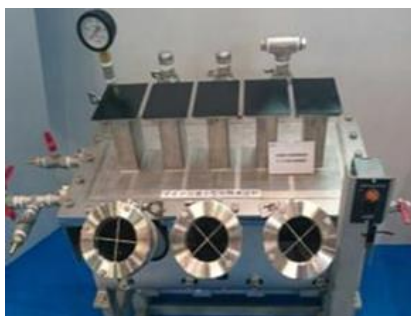
Microwave heating equipment employing GaN amplifier modules as heat sources
